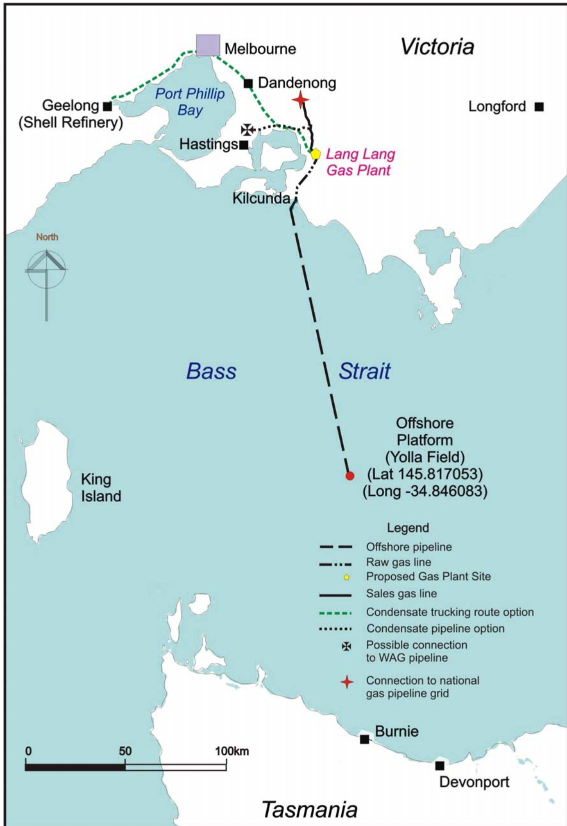
Figure 1.1: Location of the Yolla Field and major project elements
