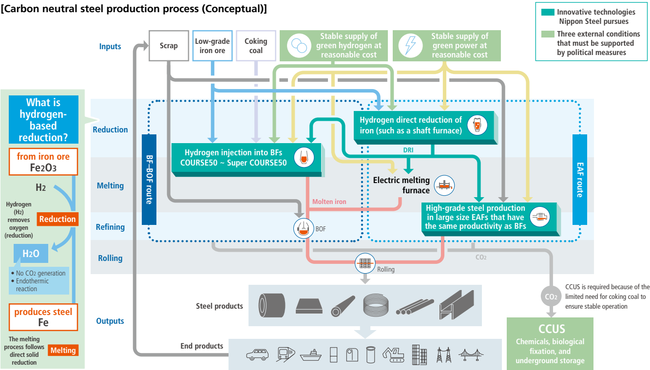
[Carbon neutral steel production process (Conceptual)]
